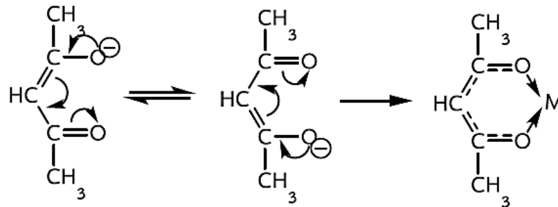
metal-acetylaceton complex (6-membered conjugate chelate rings)
