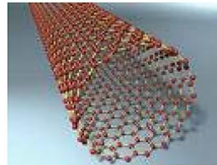
Carbon nanotube
