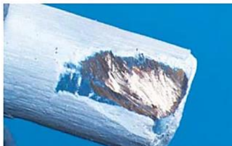
Strontium (Sr)
