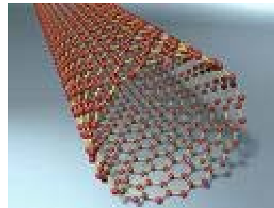
Carbon nanotube
