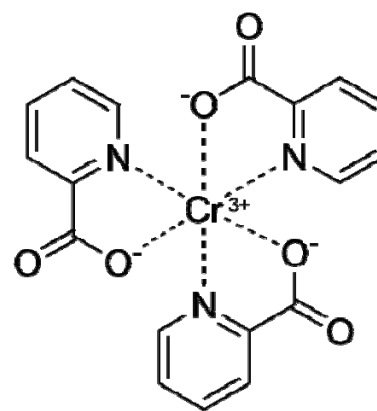
Chromium(III) picolinate
